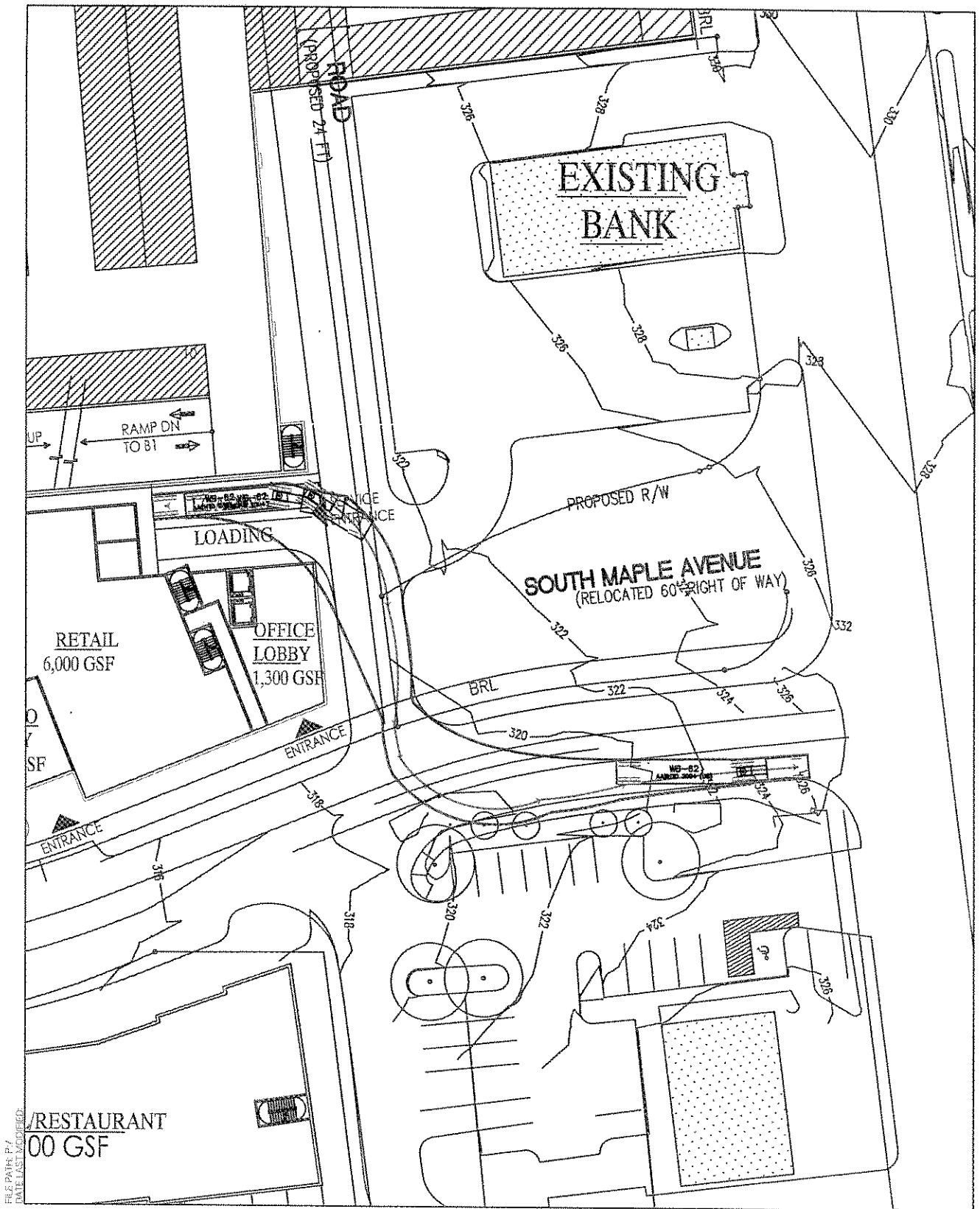
Figure 19-B WB 62 (68' Truck) Retail/Residential Loading Dock-Outbound
