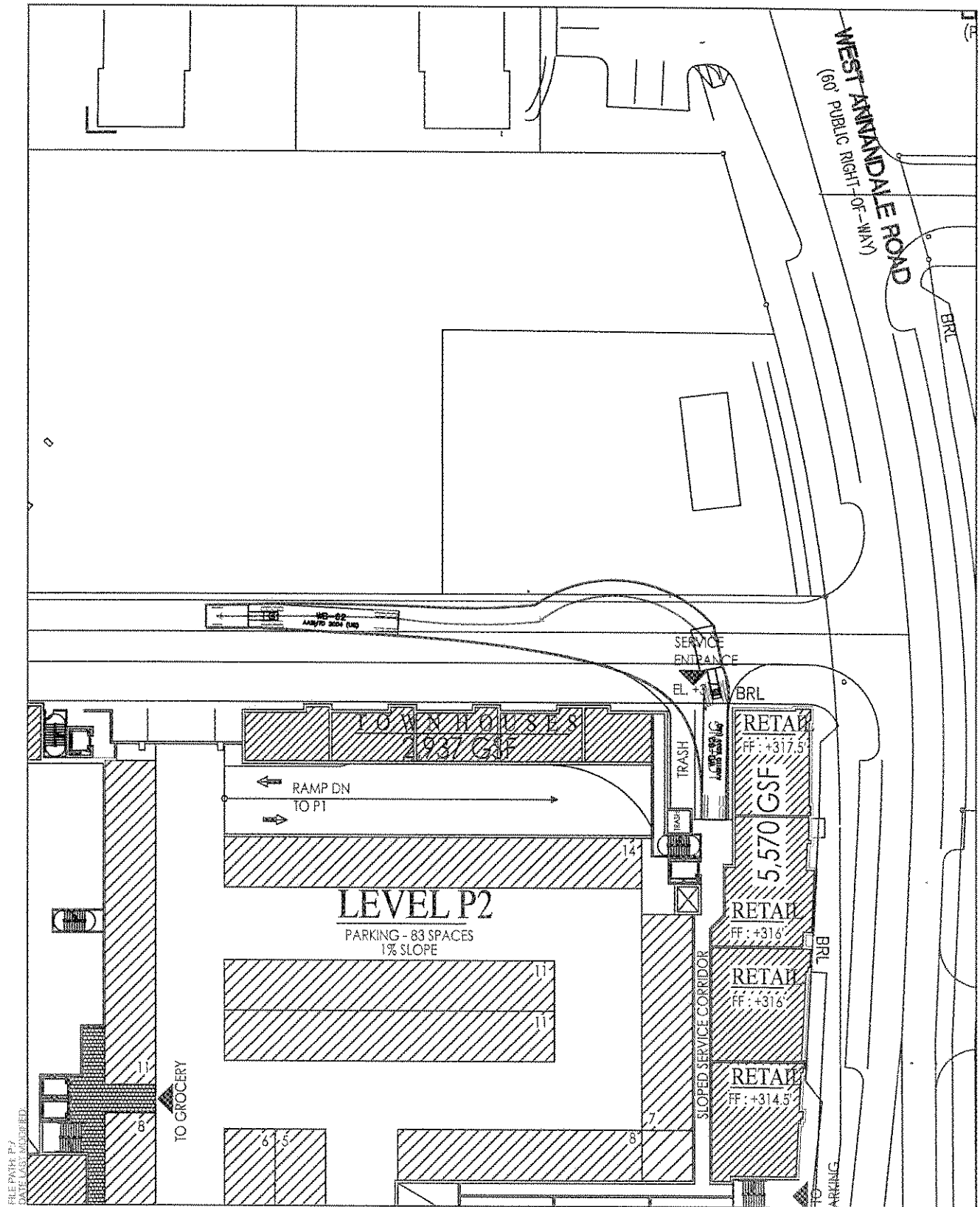
Figure 20-B WB 62 (68' Truck) Hotel Loading Dock-Outbound
