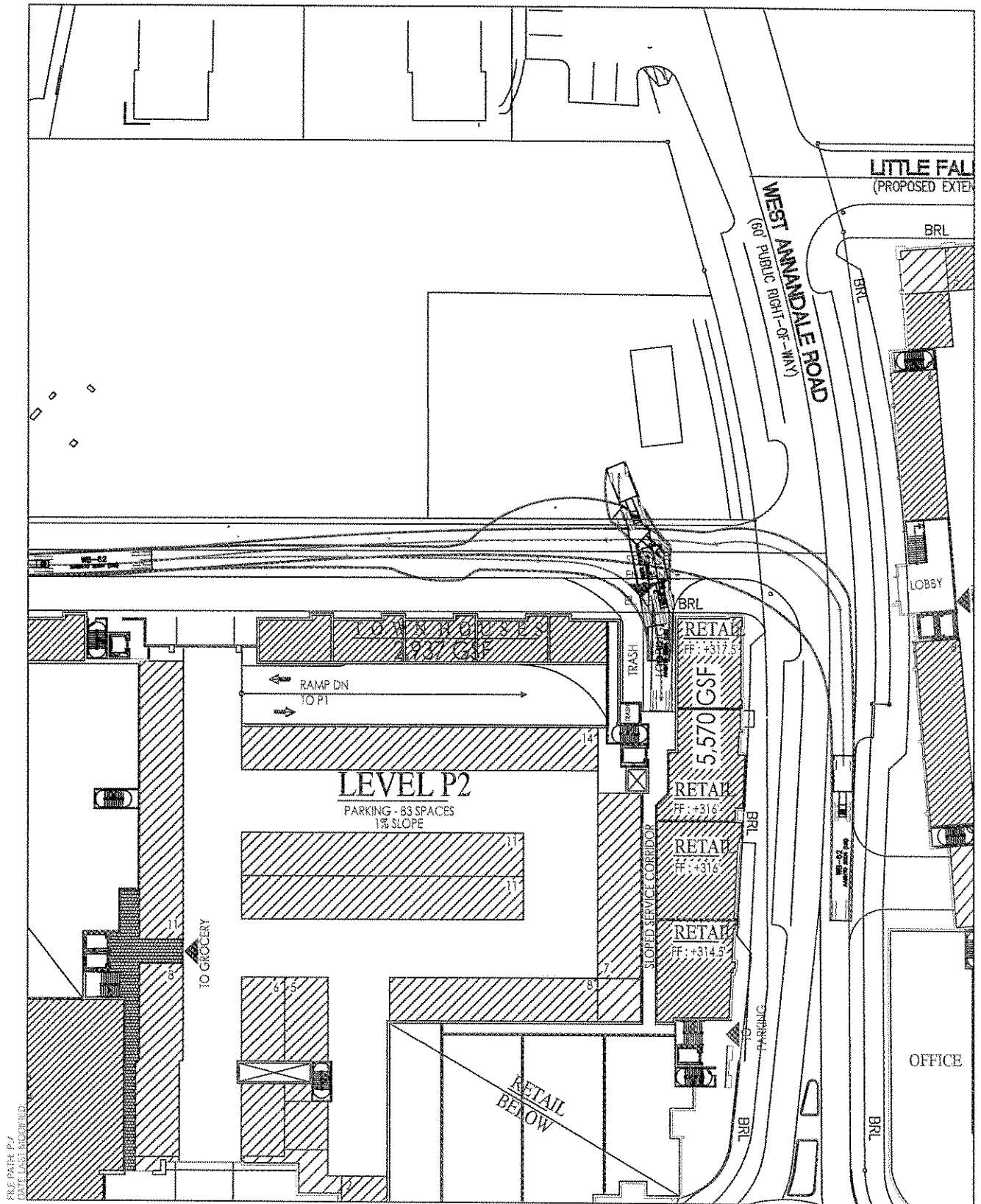
Figure 20-A WB 62 (68' Truck) Retail/Residential Loading Dock-Inbound
