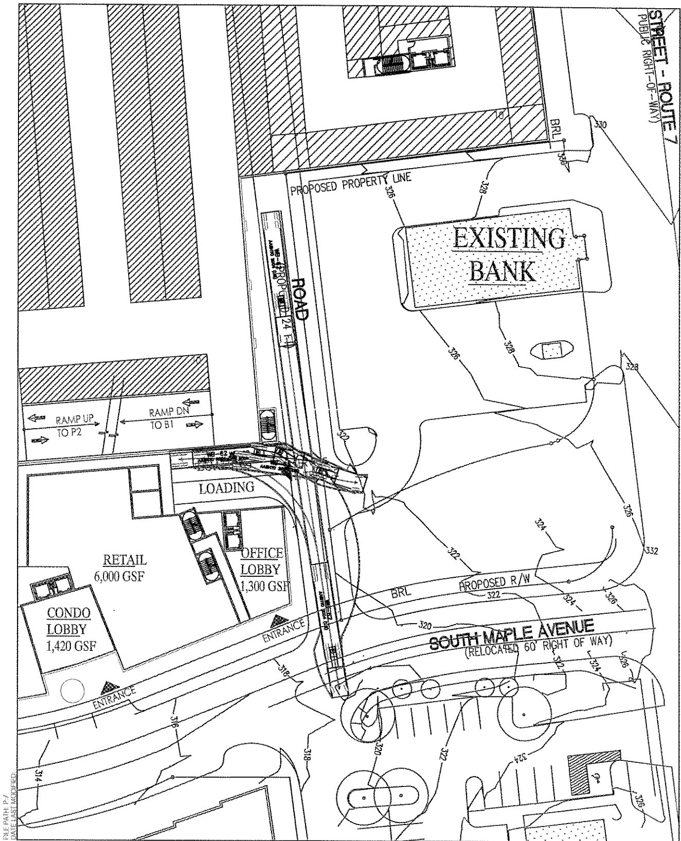
Figure 19-A WB 62 (68' Truck) Retail/Residential Loading Dock-Inbound
