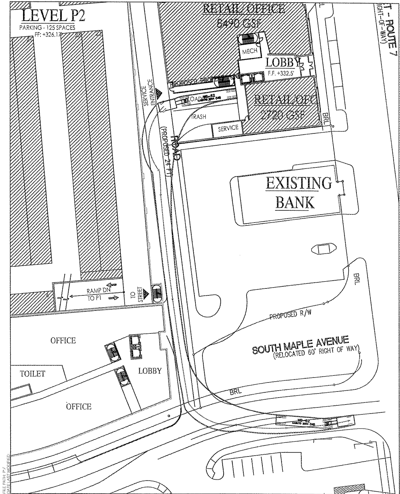
Figure 18-B WB 62 (68' Truck)v Retail Loading Dock-Outbound
