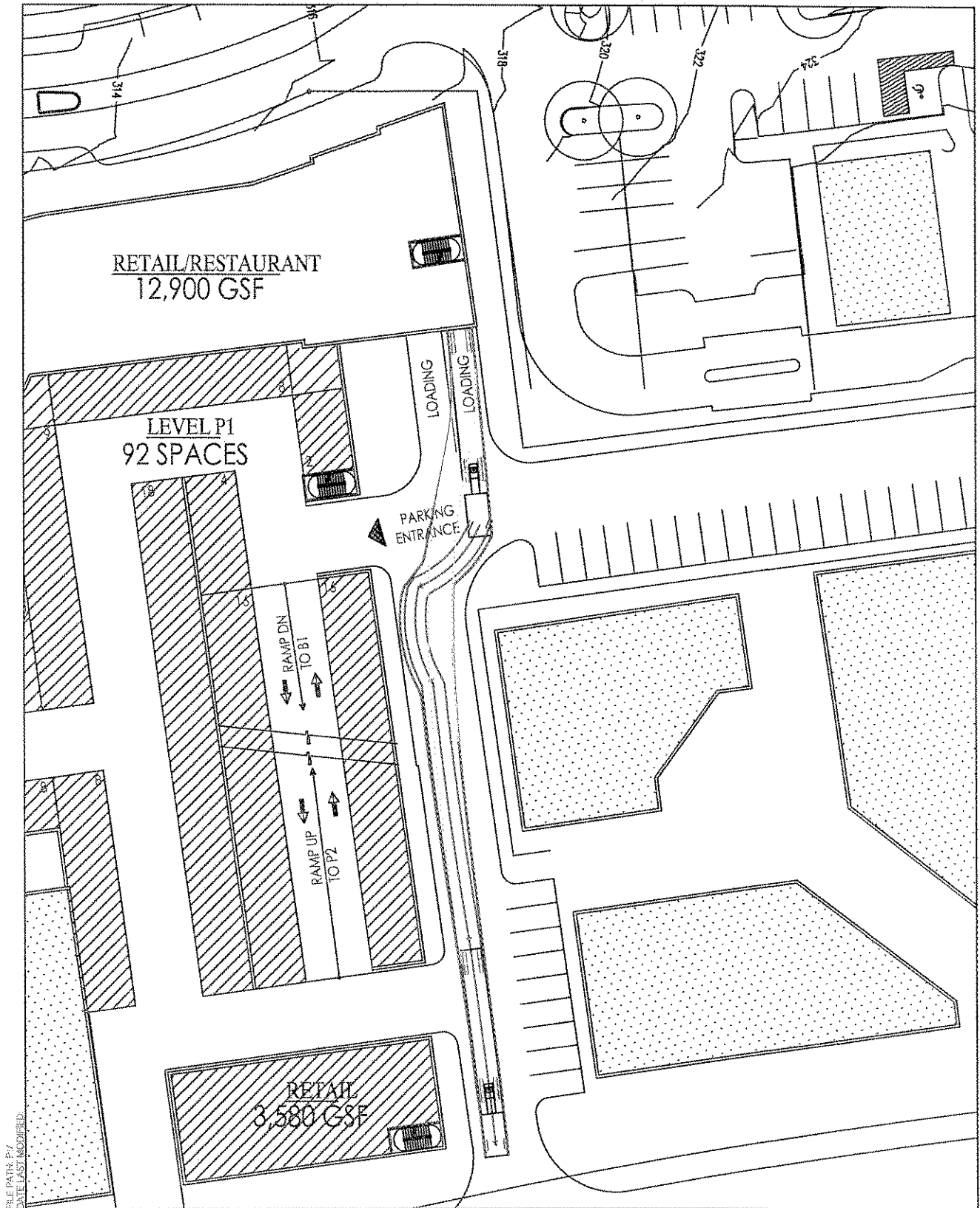
Figure 21-B WB 62 (68' Truck) Hotel Loading Dock-Outbound
