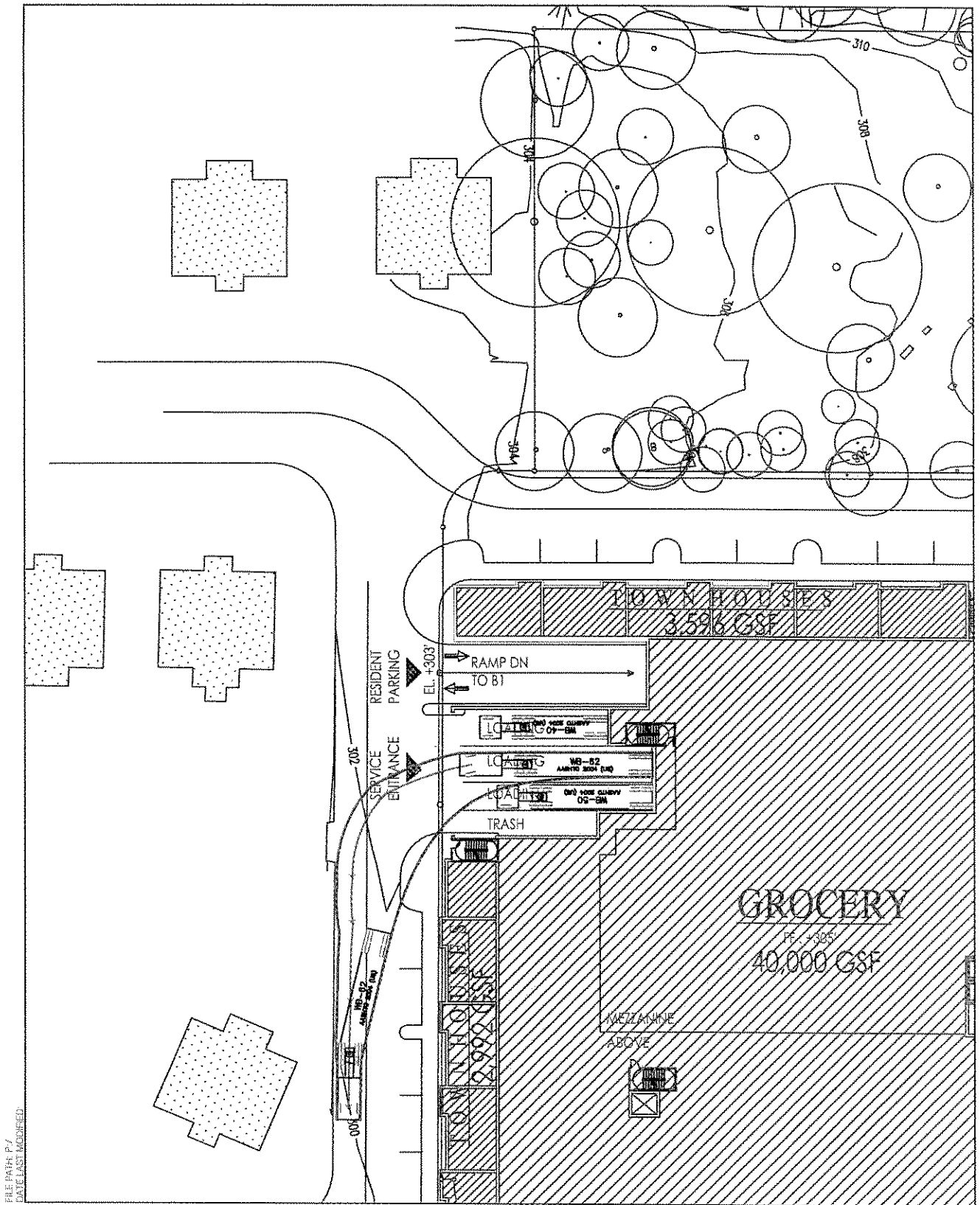
Figure 17-B WB 62 (68' Truck)v Retail Loading Dock-Outbound
