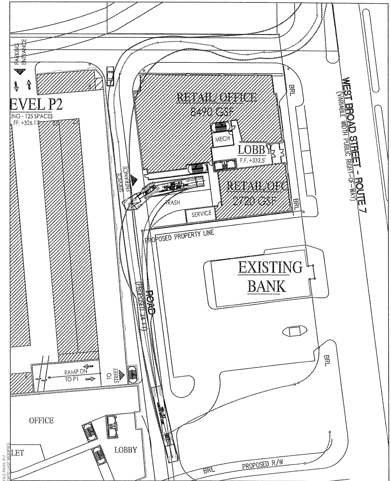
Figure 18-A WB 62 (68' Truck) Retail Loading Dock-Inbound
